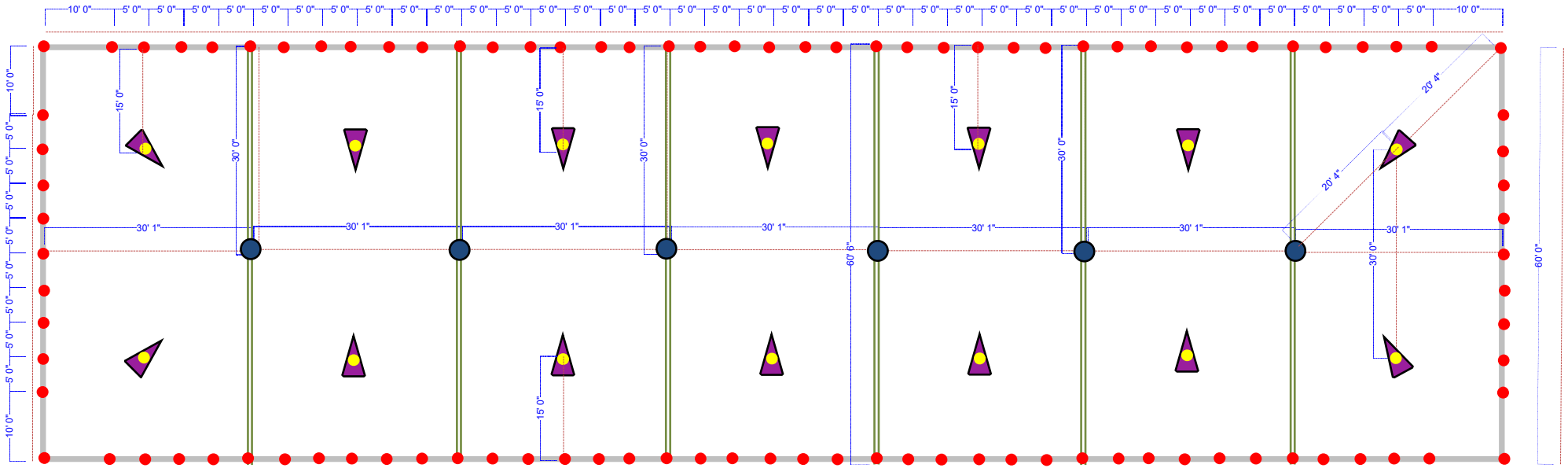
60' x 210' Pole Tent - Pole Placements
